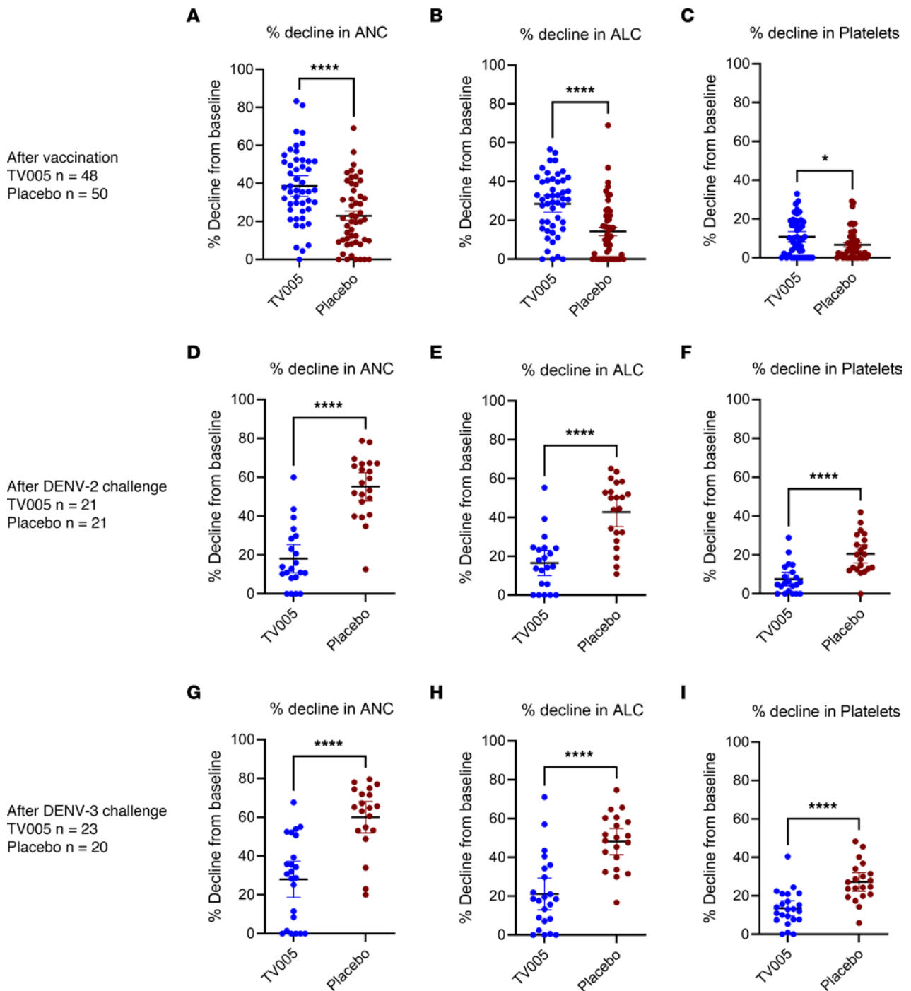
Figure 2. Decline in ALC, ANC, and platelets following administration of TV005 vaccine and DENV2 or DENV3 challenge 6 months later. Percentage of decline of the ANC, ALC, and platelet count following vaccination with TV005 compared with placebo. All TV005-vaccinated participants ( n = 48 ) and placebo recipients ( n = 50 ) from both CIR299 and CIR309 were included in these analyses. The nadir of neutrophil, lymphocyte, and platelet counts, measured through study day 16 after vaccination (or challenge), was compared with the value at study day 0 before vaccination (or before challenge). The percentage of decline was calculated as the absolute decline/baseline value \times 100 . Individual data along with means and 95% CIs are shown. An unpaired, 2-tailed Student's t test was used to compare TV005 versus placebo. (A–C) Percentage of decline of the ANC (A), ALC (B), and absolute platelet count (C) after vaccination compared with the values prior to vaccination (day 0) for volunteers who received TV005 vaccination or placebo. The percentage of decline was greater among TV005 participants than among placebo recipients (neutrophils and lymphocytes P < 0.0001 , platelets P = 0.018 ). (D–F) Percentage of decline of the ANC (D), ALC (E), and absolute platelet count (F) compared with the day of virus challenge in participants who received TV005 or placebo and who were all subsequently (6 months later) challenged with DENV2 virus. Volunteers who received placebo (not the TV005 vaccine) had significantly greater declines in neutrophils, lymphocytes, and platelets following DENV2 challenge compared with volunteers who received TV005 ( P < 0.0001 ). (G–I) Percentage of decline of the ANC (G), ALC (H), and absolute platelet count (I) compared with the day of viral challenge in participants who received TV005 or placebo and who, 6 months later, all received DENV3 virus challenge. Volunteers who received placebo (not TV005 vaccine) had significantly greater declines in neutrophils, lymphocytes, and platelets following DENV3 challenge compared with volunteers who received TV005 ( P < 0.0001 ). * P < 0.05 and **** P < 0.0001 , by unpaired, 2-tailed Student's t test (A–I).
