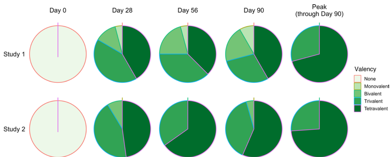
Figure 3. Seroconversion to multiple serotypes following vaccination of dengue-naive adult volunteers with TV005. Following TV005 vaccination of adult dengue-naive volunteers (day) and at subsequent time points after vaccination, volunteers demonstrated seroconversion to 1 (monovalent) to 4 (tetravalent) serotypes. The majority of participants in study 1 (CIR299) and study 2 (CIR309) demonstrated seroconversion to all 4 (trivalent) serotypes.
