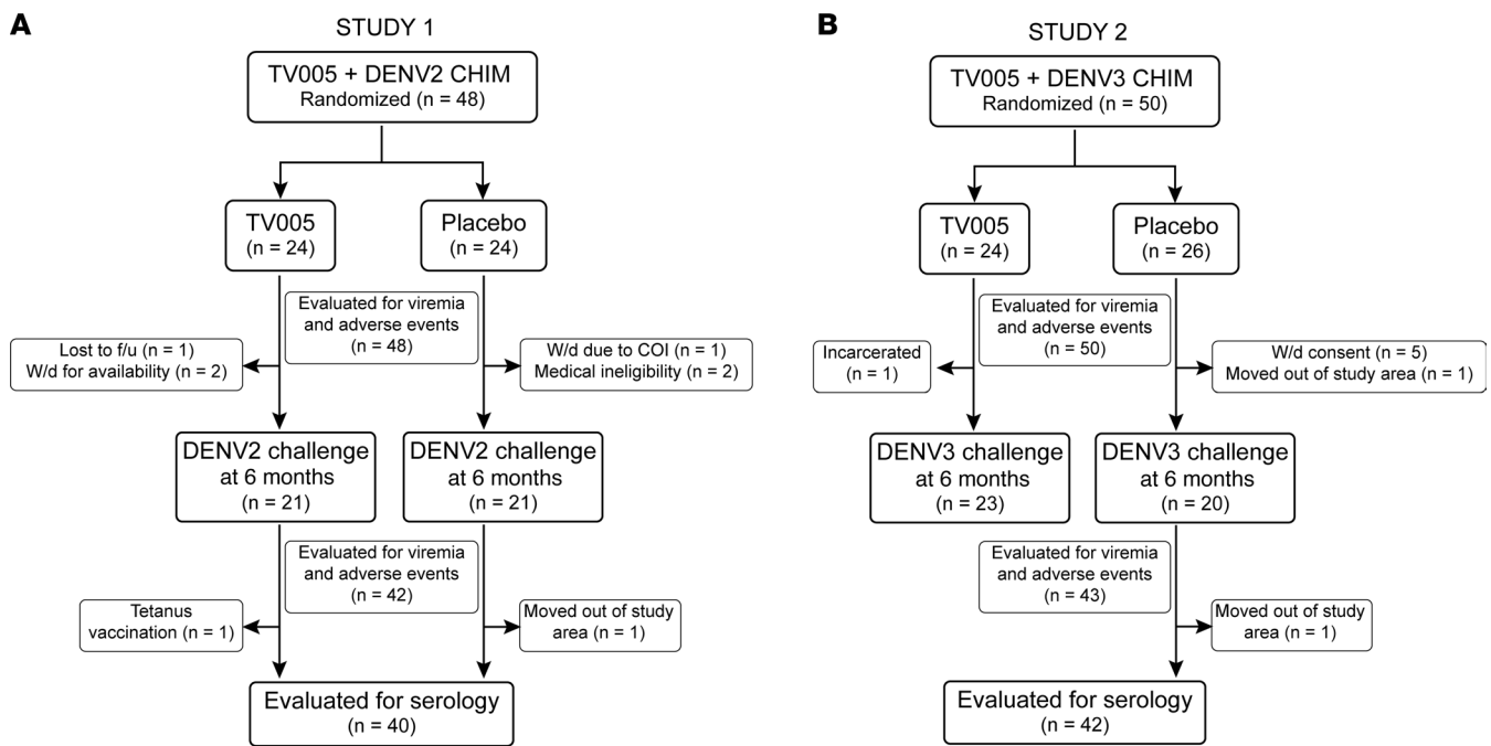
Figure 1. CONSORT diagrams of enrollment, retention, and interventions. (A) Study 1 (CIR299) is a placebo-controlled trial of the efficacy of TV005 against rDEN2 \Delta 30 challenge. (B) Study 2 (CIR309) is a placebo-controlled trial of the efficacy of TV005 against rDEN3 \Delta 30 challenge. COI, conflict of interest; f/u, follow-up; W/d, withdrew.
