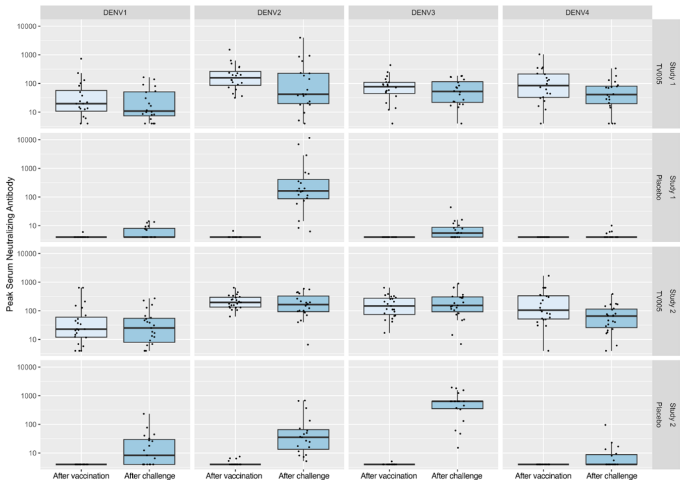
Figure 4. Serum neutralizing antibody responses through day 90 in TV005 vaccine or placebo recipients, following TV005 vaccination and subsequent DENV2 or DENV3 virus challenge. Individual data are shown along with box and whisker plots; the box is the median with 25th and 75th percentiles; whiskers extend to the minimum/maximum values, no further than 1.5 times the IQR from the lower/upper quartile. For DENV2 responses, all data shown after vaccination and challenge reflect responses to the rDEN2/4Δ30 (NGC) strain. Responses to both the rDEN2Δ30 (NGC) and rDEN2Δ30 strain (Tonga) are shown in Table 10.
